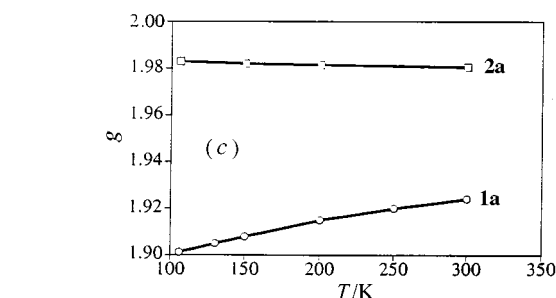
Fig. 7 Powder ESR spectra for complex 1a : (a) evolution within the 105–300 K temperature range, (b) experimental and simulated (dotted line) ESR spectra at 105 K, (c) temperature dependencies of the g factor for 1a and 2a
