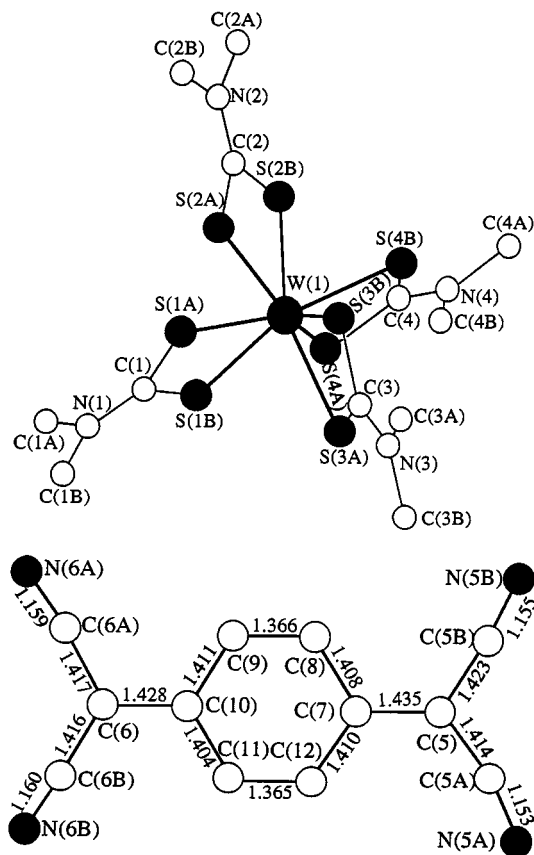
Fig. 2 The cation and anion in complex 1a : atom numbering and TCNQ bond lengths ( \text{\AA} , e.s.d.s in the least significant digits (7), (8) or (9). W-S bond lengths (e.s.d.s in the least significant digits): W-S(1B) 2.491(6) , W-S(2B) 2.494(6) , W-S(2A) 2.511(6) , W-S(1A) 2.532(6) , W-S(4B) 2.503(6) , W-S(3B) 2.508(6) , W-S(4A) 2.542(6) , W(1)-S(3A) 2.553(6)
